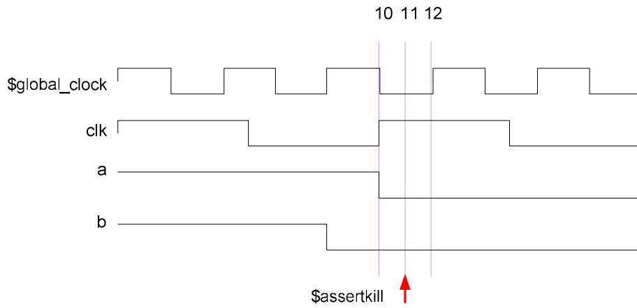
Figure 38-1: Assertions with global clocking future sampled value functions (Editor to assign a correct number)
